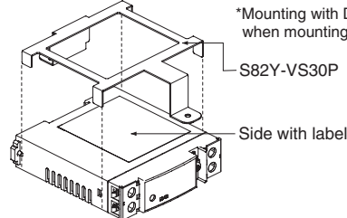
Mounting facing horizontally with S82Y-VS30P*
