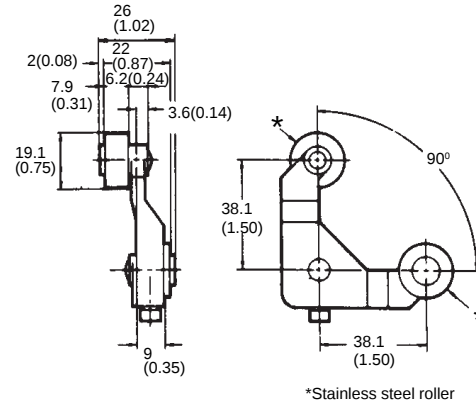
D4A-E10 Fork Roller Lever (Left roller back/Right roller front)
