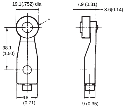
D4A-A00 Standard Roller
