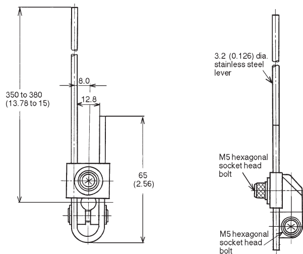
WL-3A100 Adjustable Rod Lever
